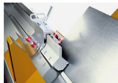
Autopilot and reinforced seaming bar on the RAS 20.12 DuctZipper.
