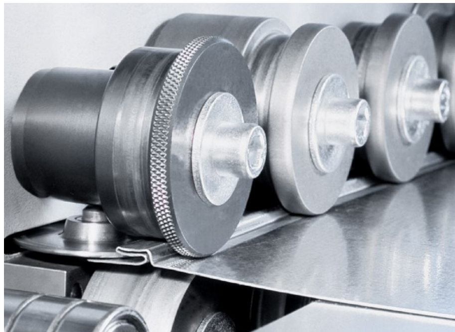
Set of rolls for Pittsburgh seam
